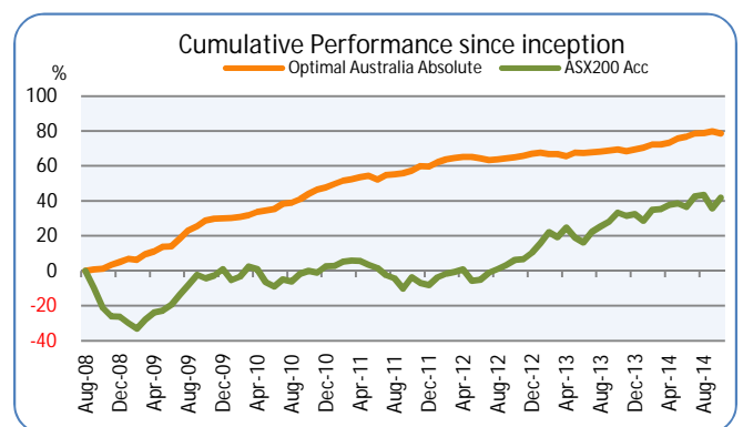
Chart 1: Cumulative Returns
